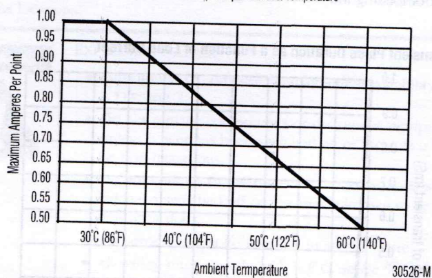
1769-OB32 Maximum Amperes per Point vs. Temperature
