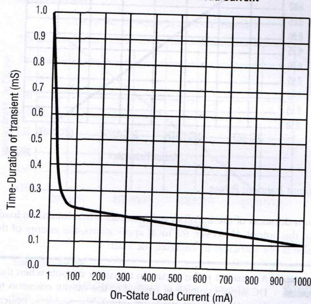
Transient Pluse Duration as a Function of Load Current
